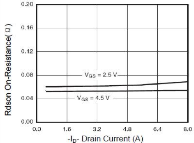
Figure 6 Drain-Source On-Resistance
